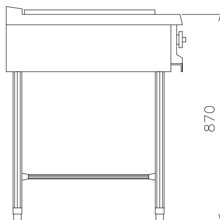
Lateral
